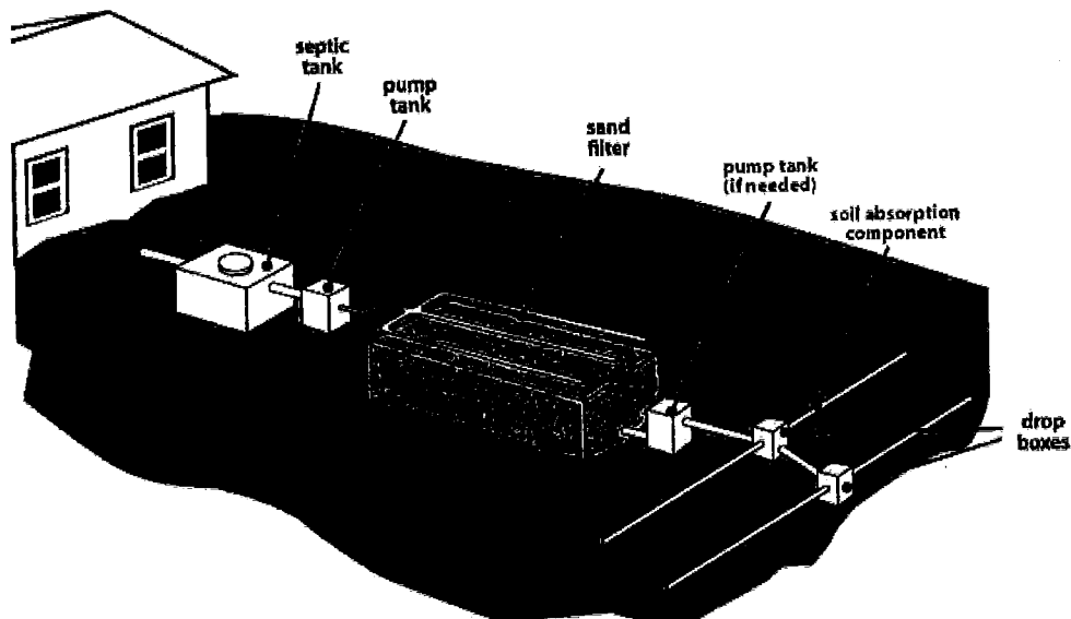
Figure 1. Time Dosed Sand Filter
