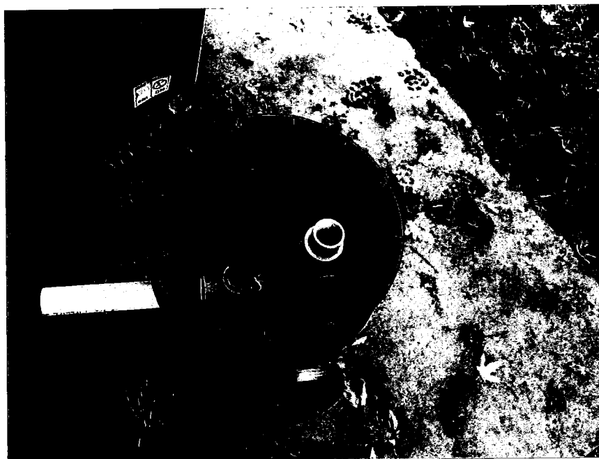
Figure 8. Turn-up and \frac{3}{4} inch air gap/ bleeder at the end of each lateral for routine maintenance
